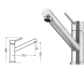
Swivel mixer Maximum pressure / 500kpa
