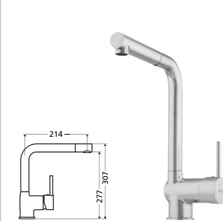
Pull out right angle mixer Maximum pressure / 500kpa
