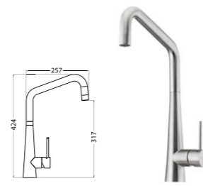
Square goose neck mixer Maximum pressure / 500kpa
