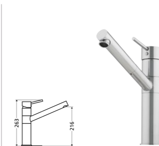
Swivel mixer Maximum pressure / 500kpa
