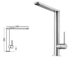
Right angle mixer Maximum pressure / 500kpa
