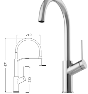
Goose neck mixer Maximum pressure / 600kpa
