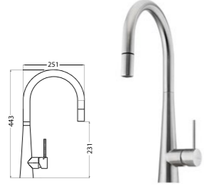
Goose neck pull out mixer Maximum pressure / 500kpa
